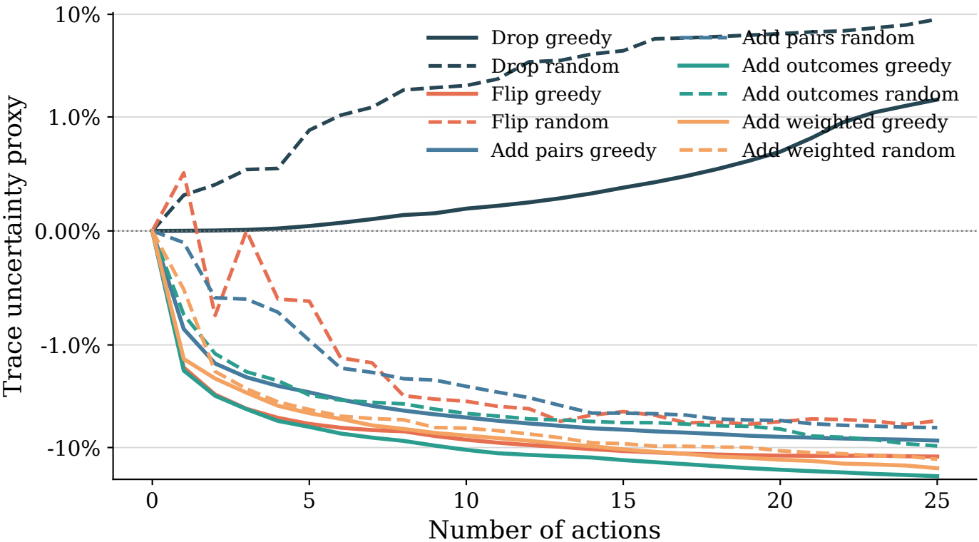
ATP Top-10 Matchups (2020-2024): trace uncertainty proxy vs actions
