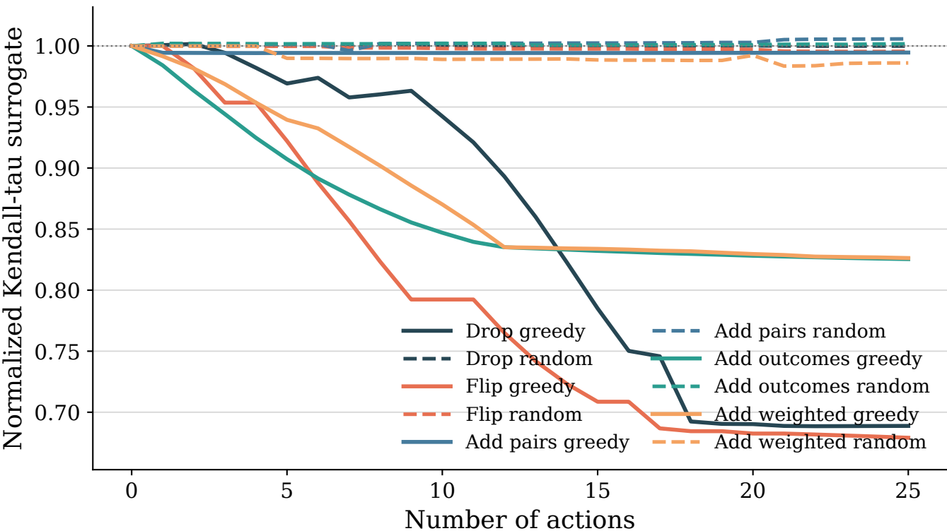
WebDev Arena: Kendall tau vs actions
