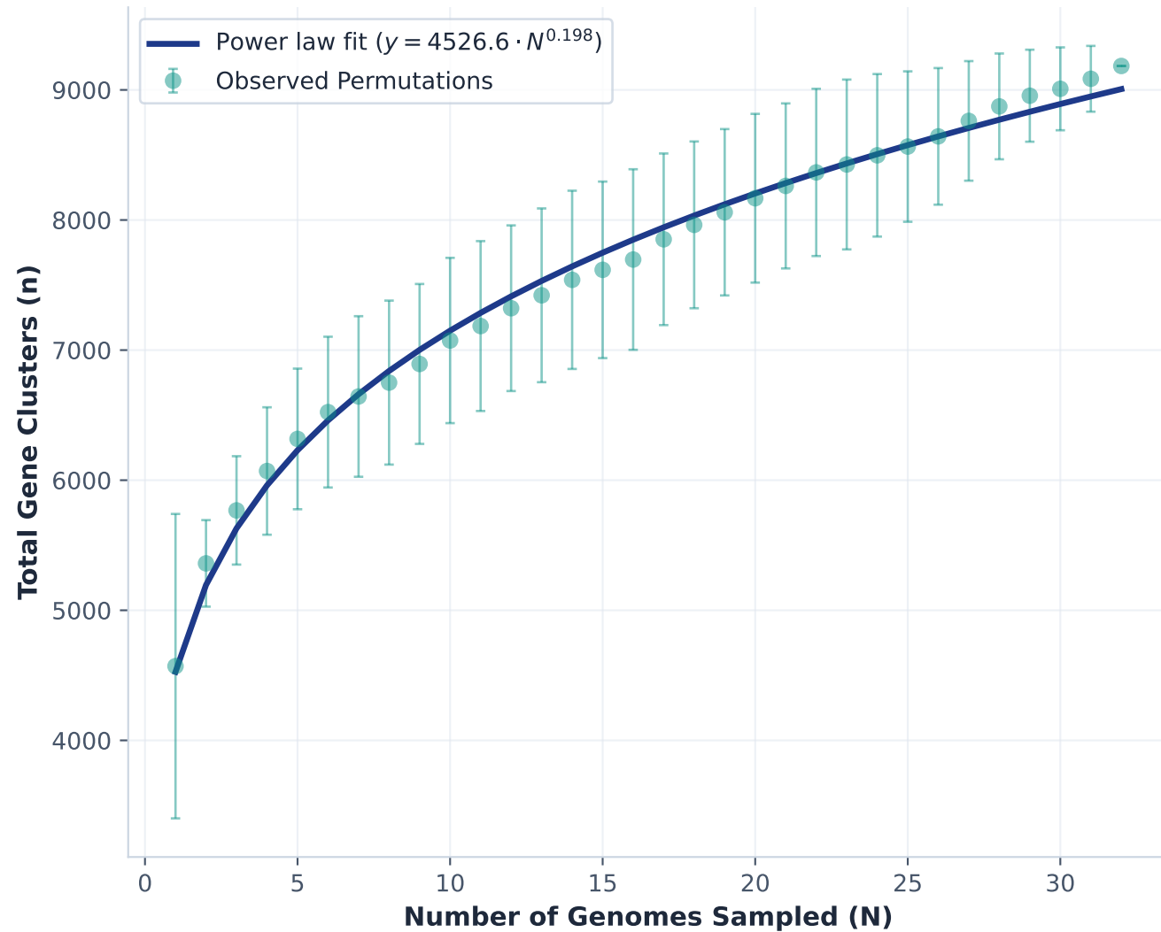
A) Pangenome Accumulation Curve
