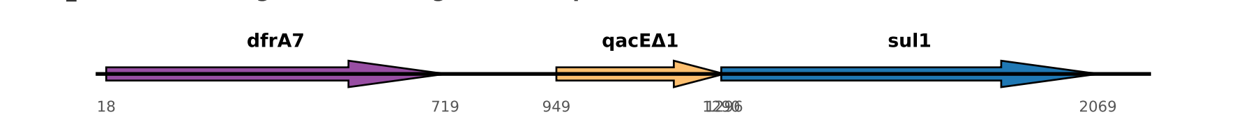
NODE_41 (Class 1 Integron 3'-CS, Length: 2,175 bp)
