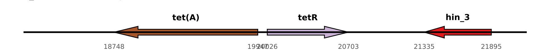
NODE_30 (tet locus, Region shown: 18,000-22,184 bp)
