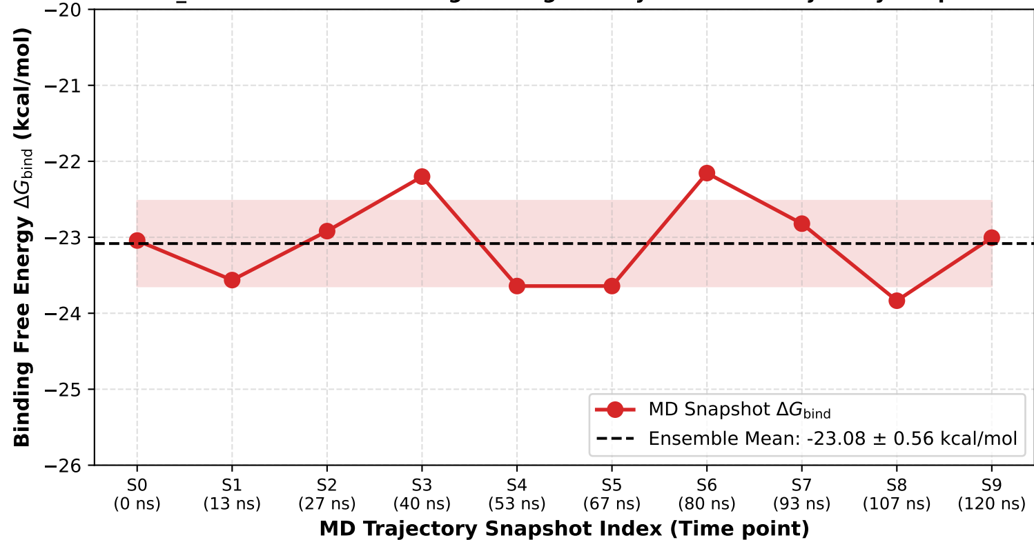
GNAT_KA27 Ensemble Docking Binding Affinity Across 10 Trajectory Snapshots
