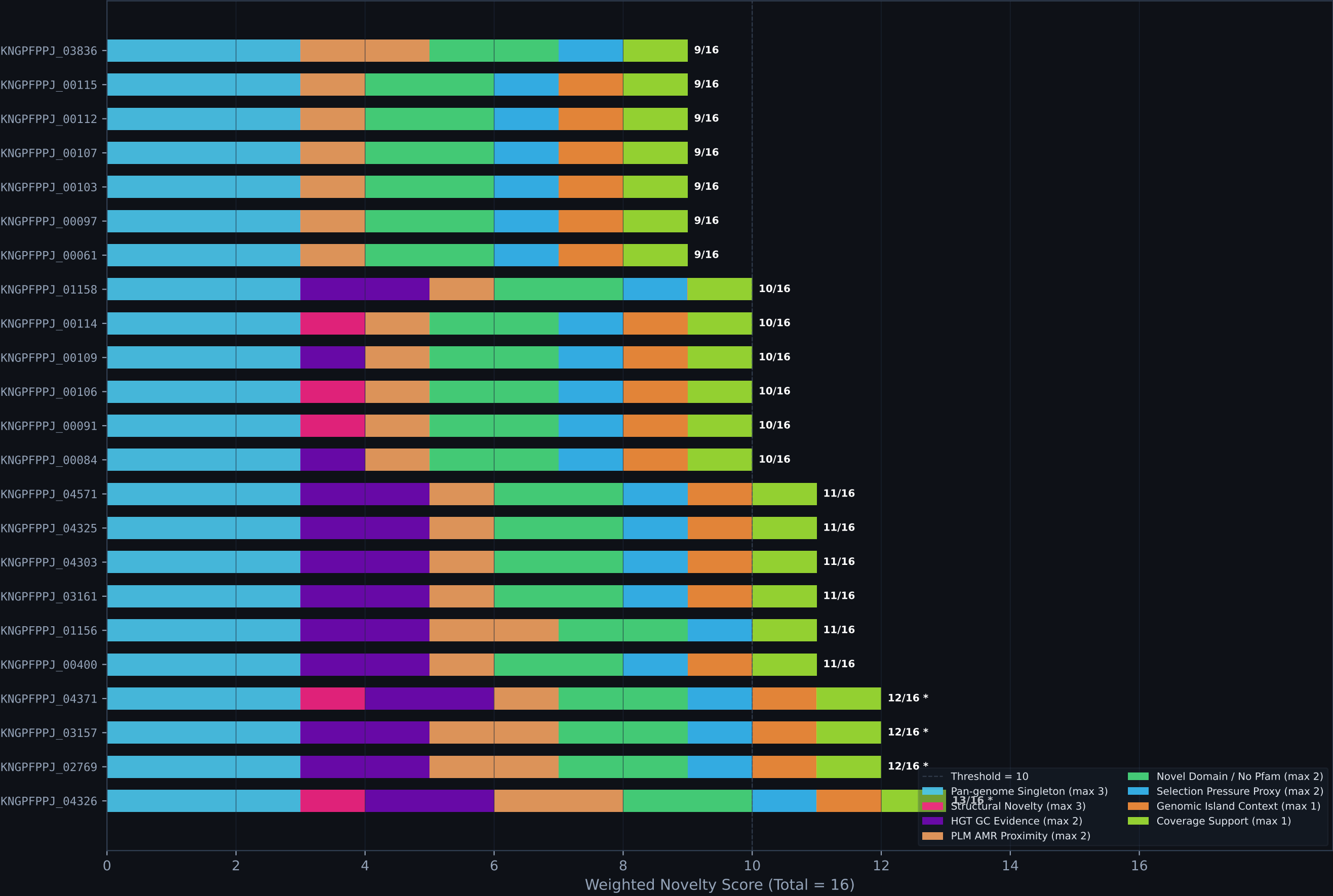
Figure 10 — Weighted Novelty Score for 23 Novel Gene Candidates (QA5221 E. coli Isolate)
