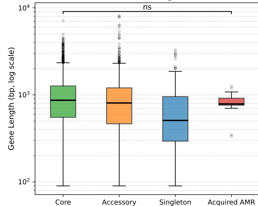
C) Gene Length
