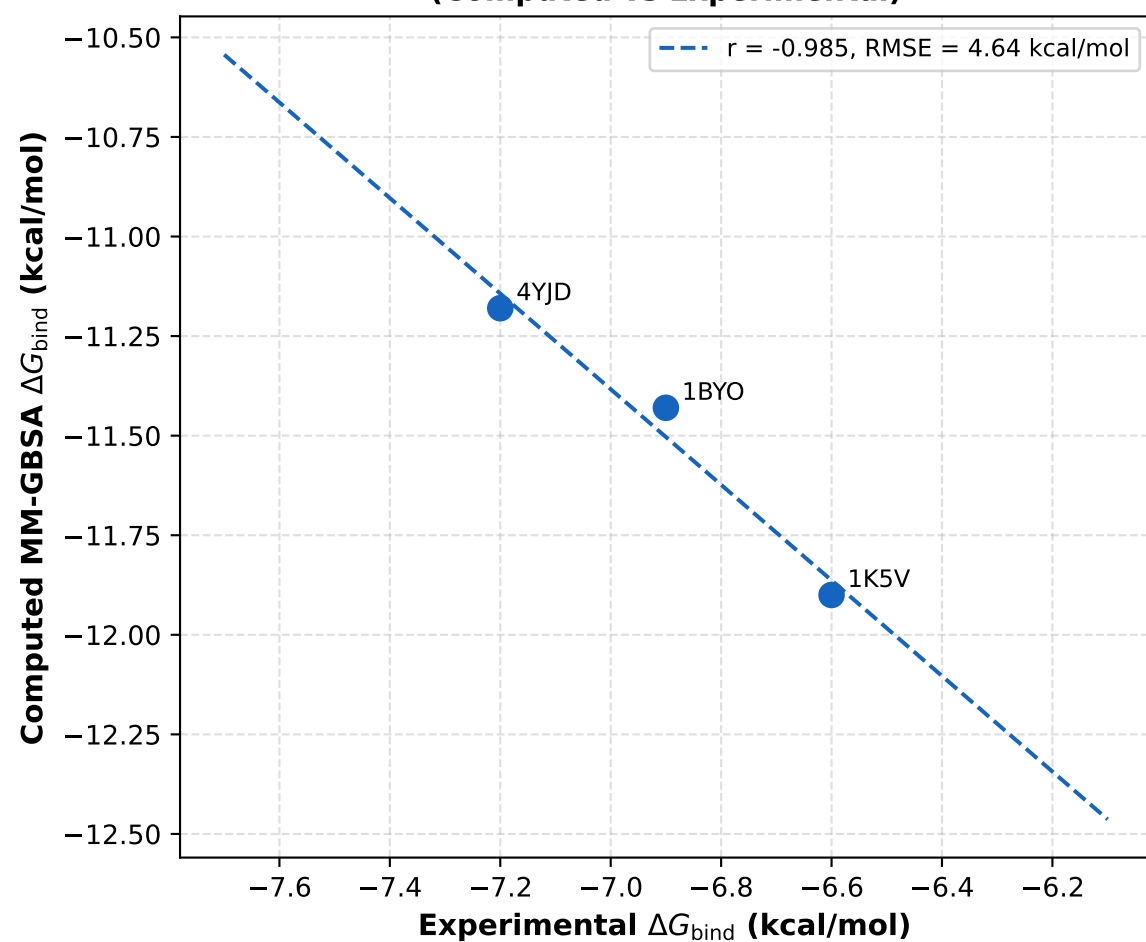
(b) Protocol Validation (Computed vs Experimental)
