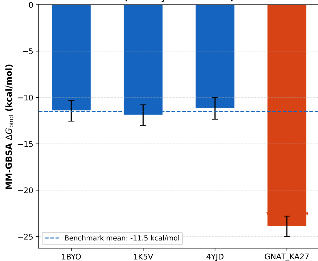
(a) Computed vs Benchmark GNAT Complexes (Kanamycin Substrate)
