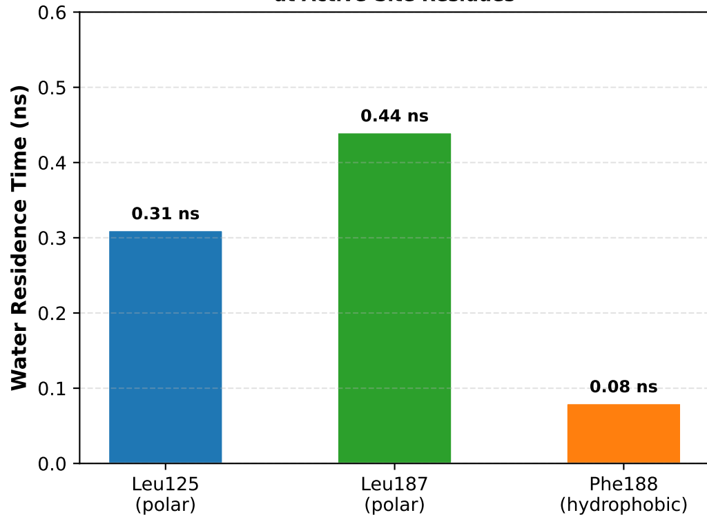
(b) Water Residence Times at Active-Site Residues
