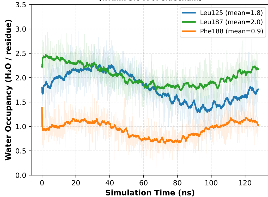
(a) Active-Site Water Occupancy (within 3.5 Å of sidechain)
