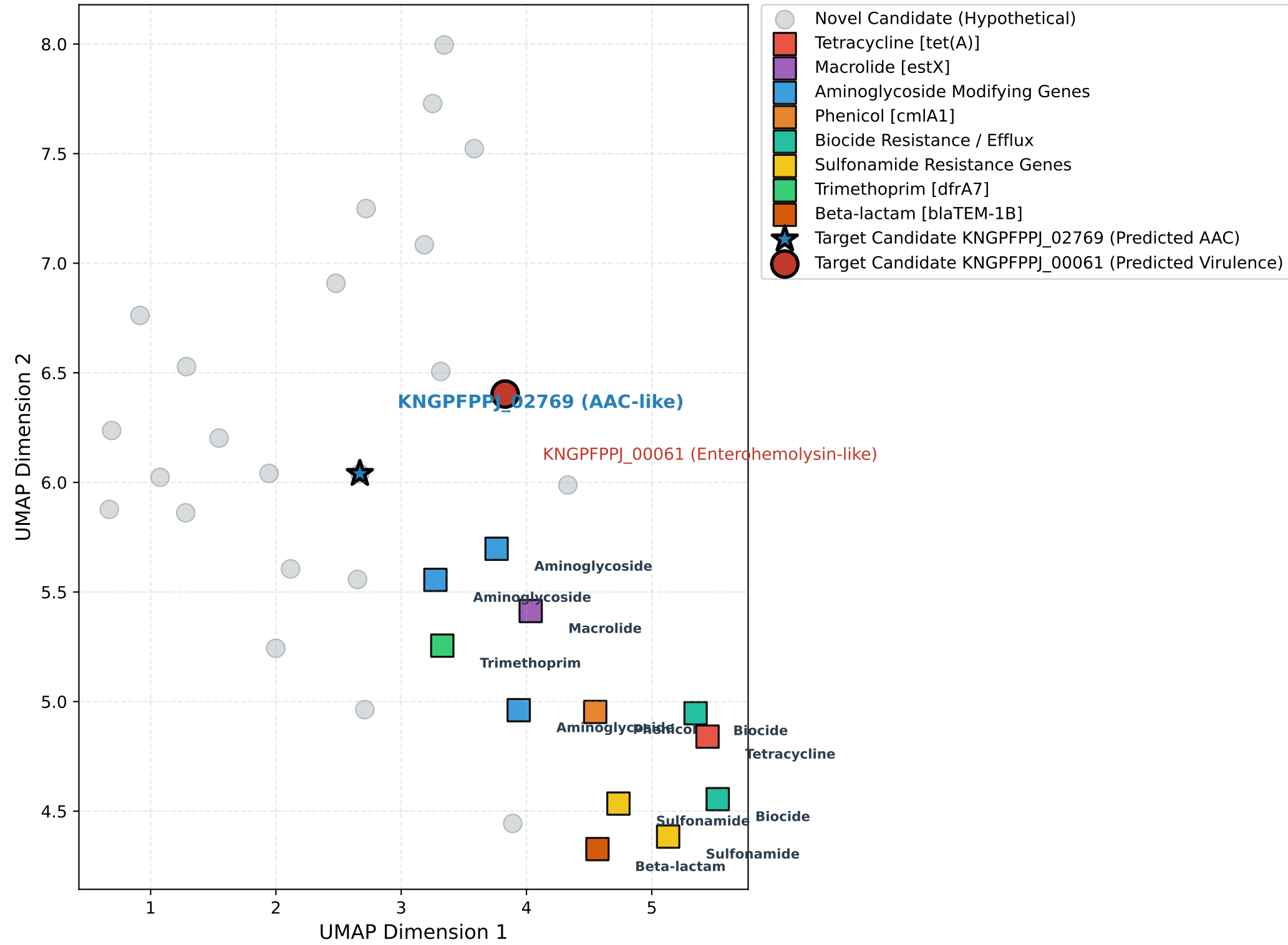
Figure 9: Protein Language Model (ESM-2) Embedding Space UMAP Clustering
