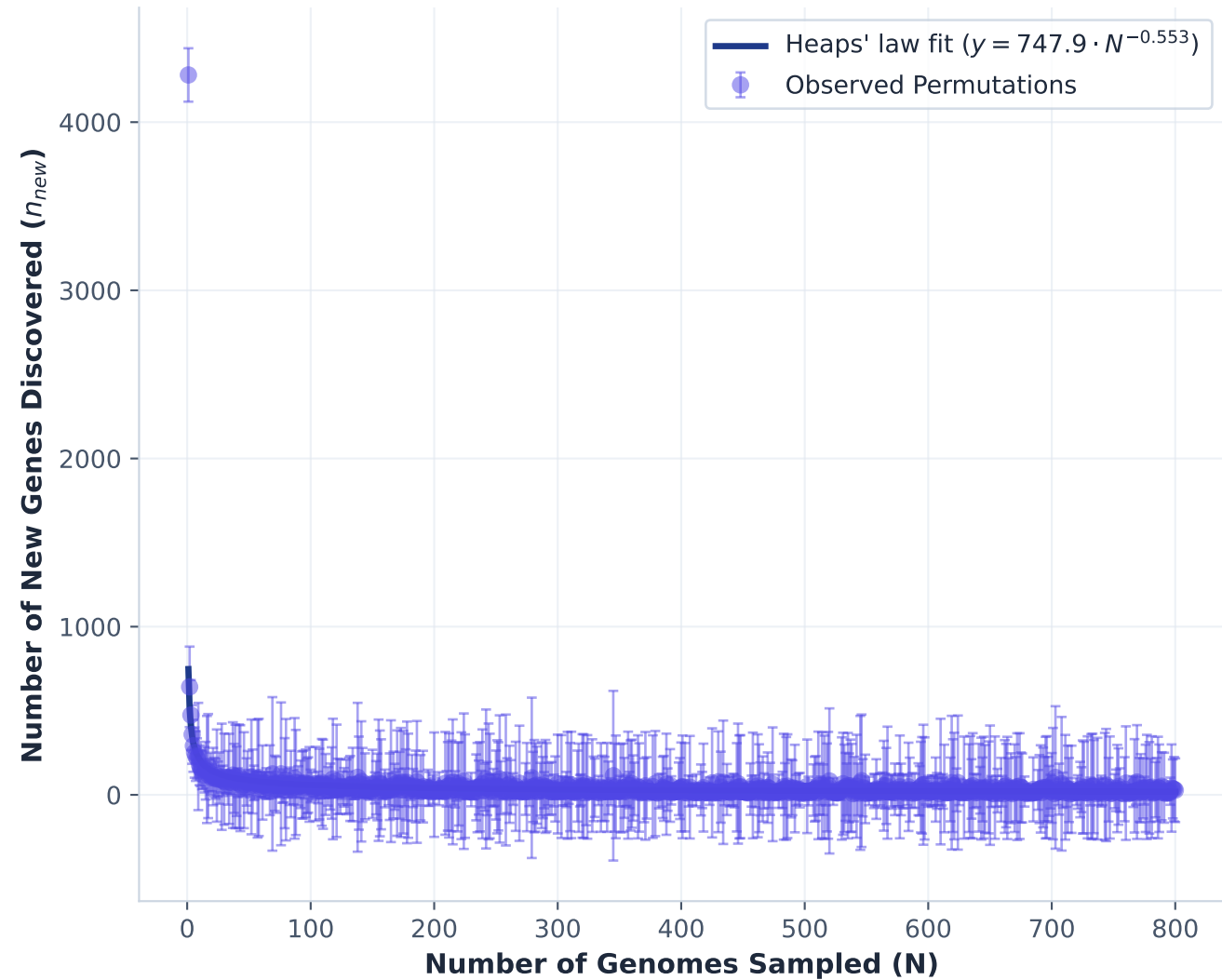
B) New Genes Discovery Curve
