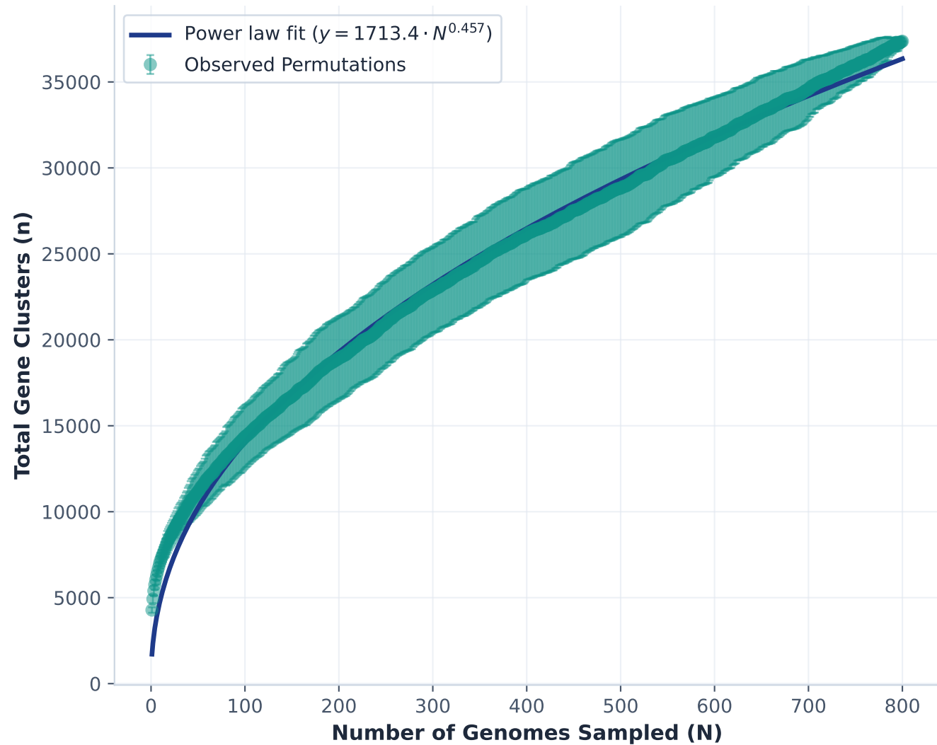
A) Pangenome Accumulation Curve
