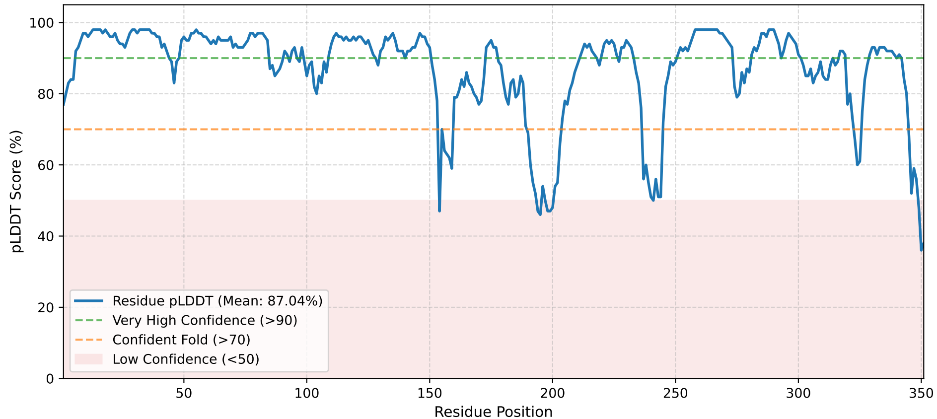
ESMFold Prediction Confidence (pLDDT) per Residue for KNGPFPPJ_02769
