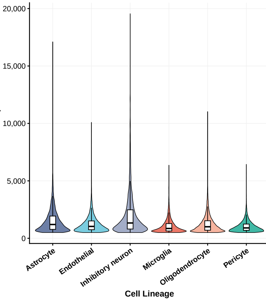
Total UMI Counts per Nucleus
