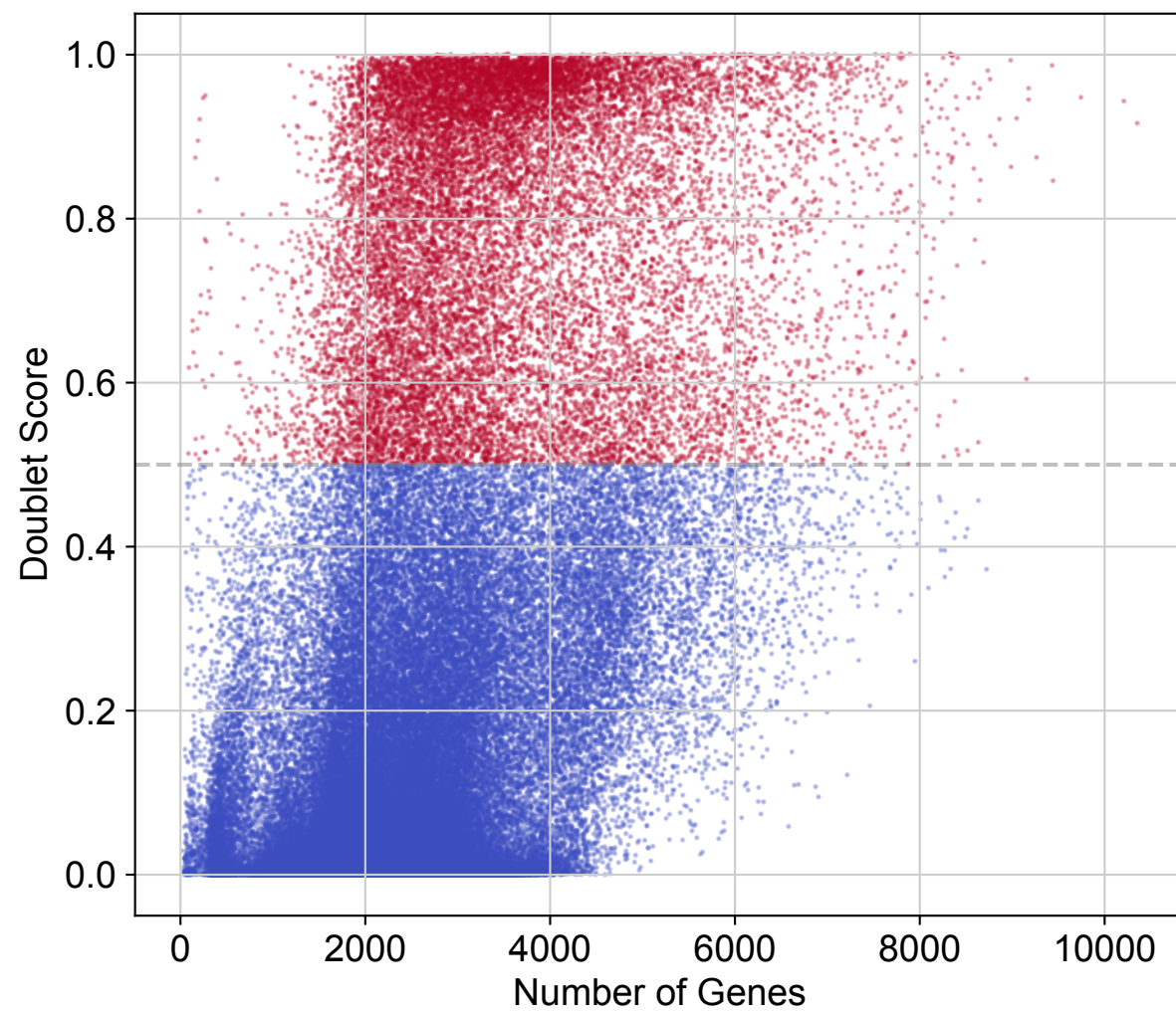
Score vs Gene Count
