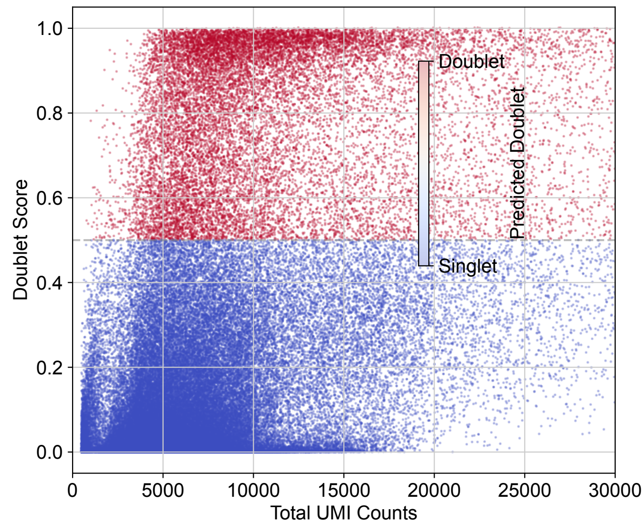
Score vs UMI Count
