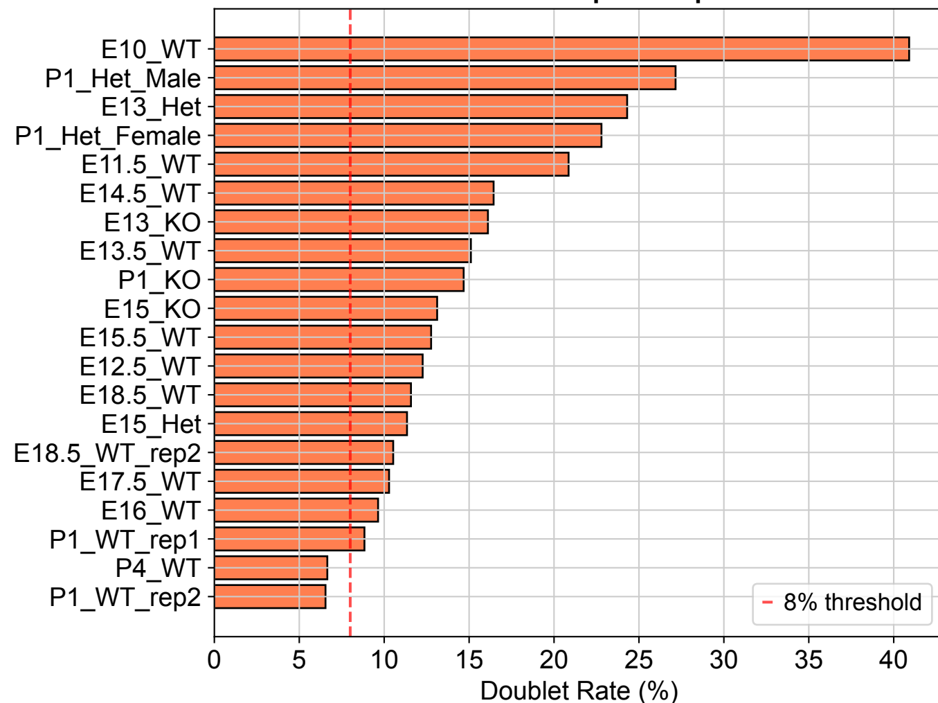
Doublet Rate per Sample
