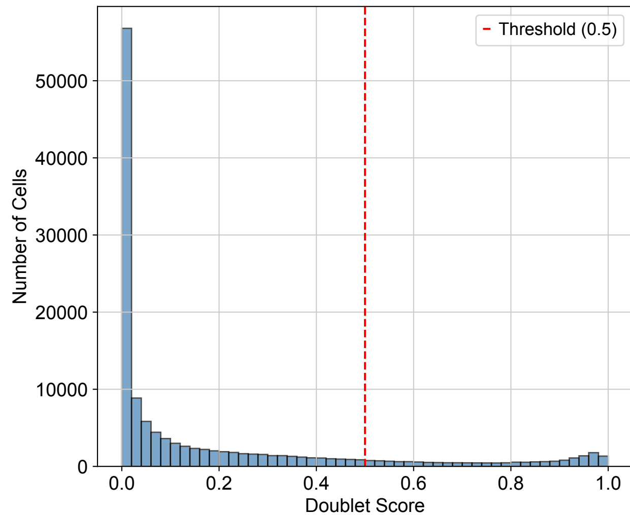
Doublet Score Distribution
