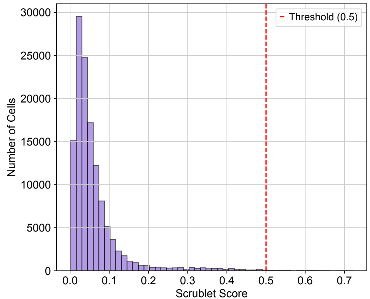
Scrublet Score Distribution
