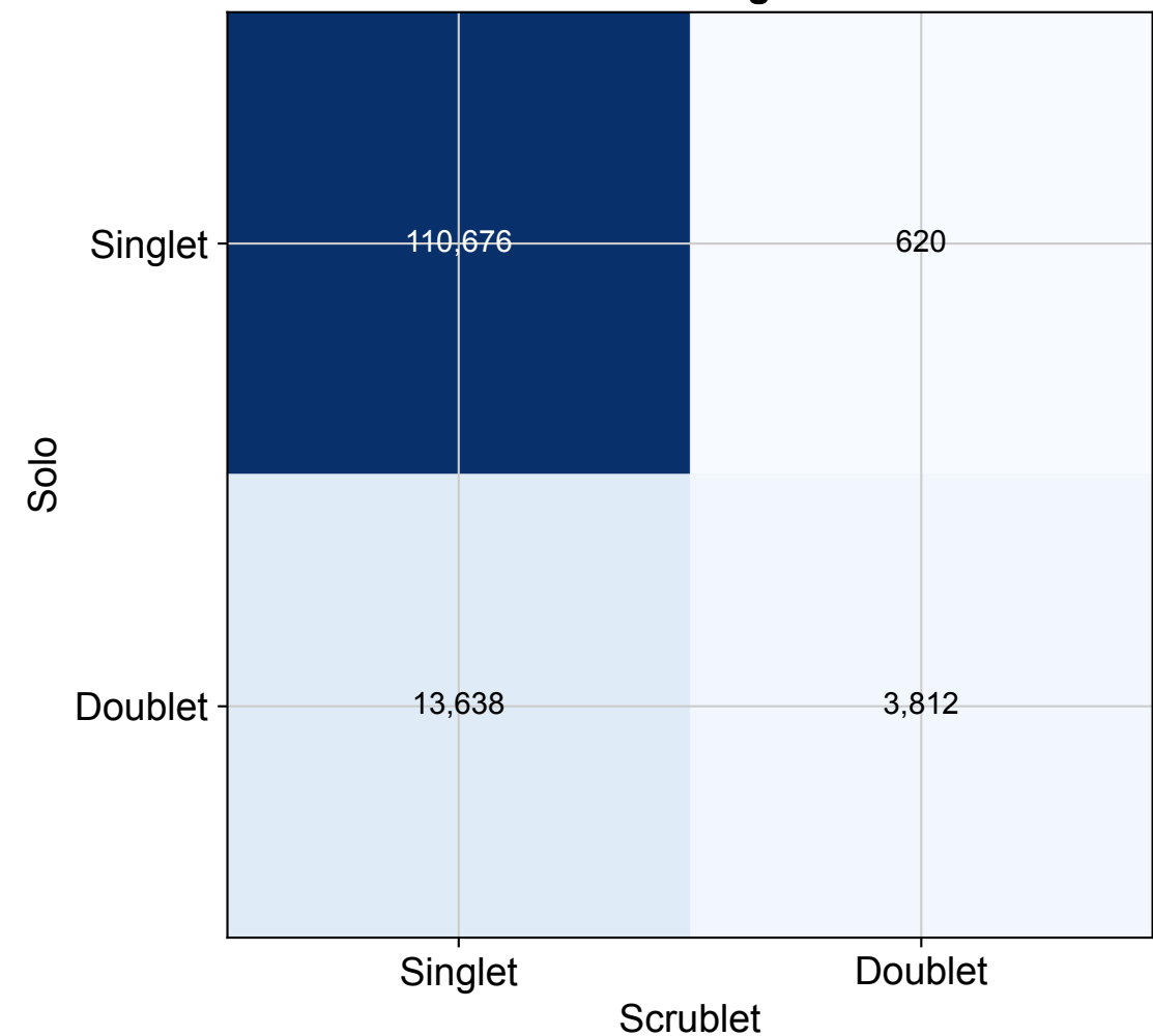
Classification Agreement
