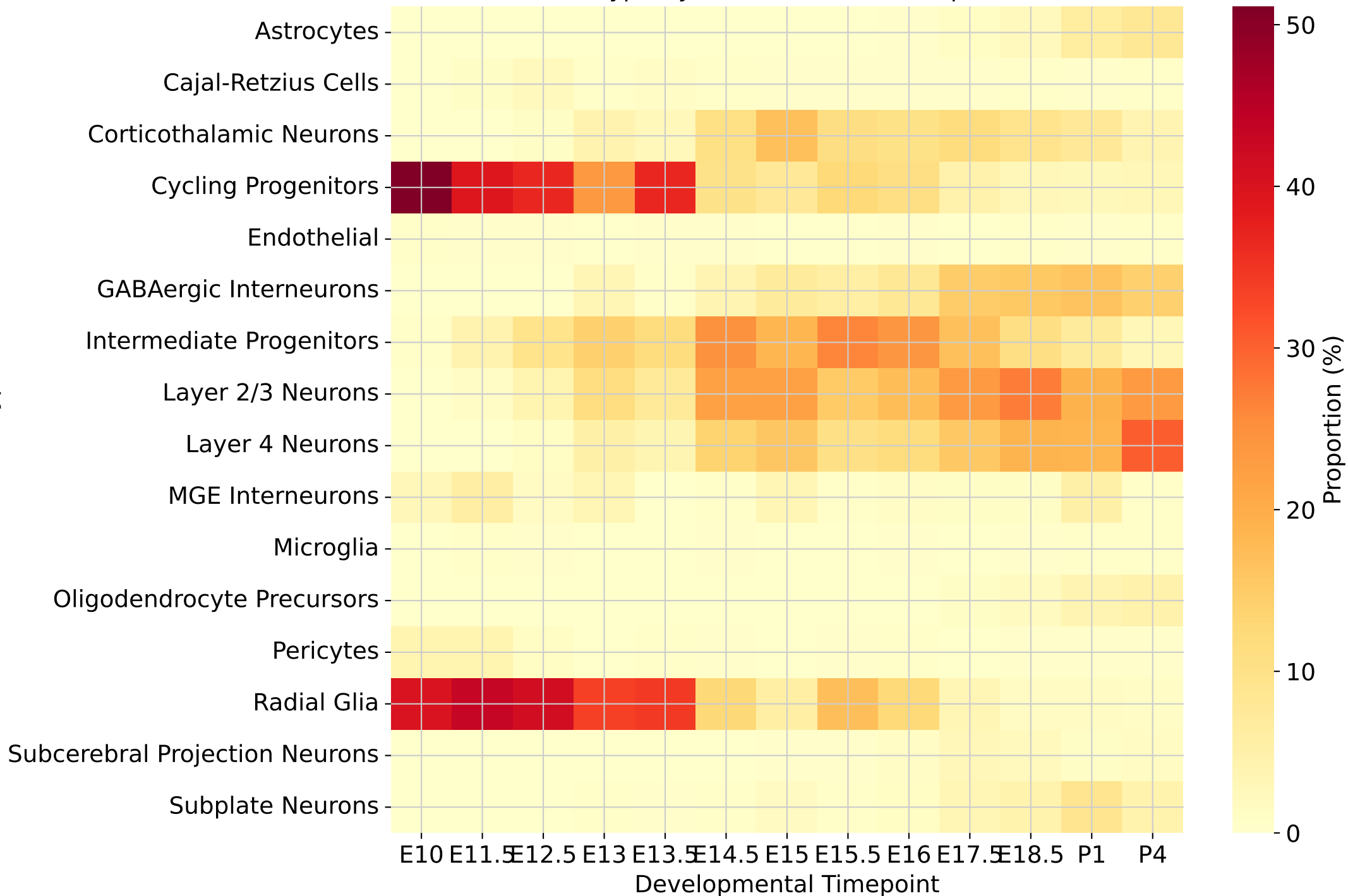
Cell Type Dynamics Across Development
