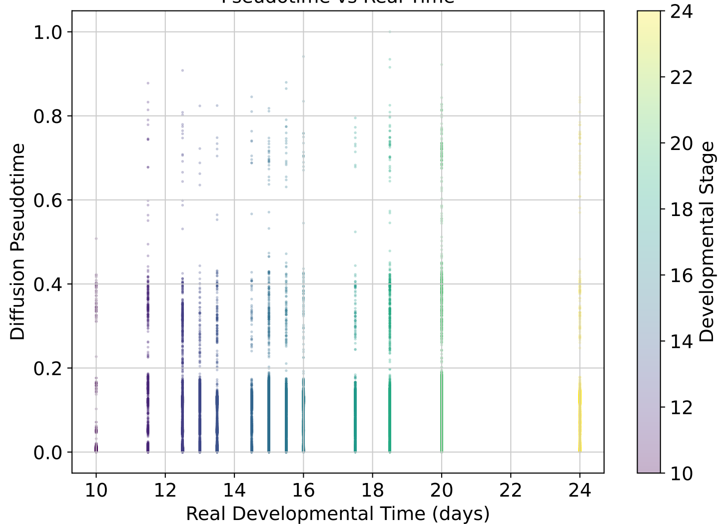
Pseudotime vs Real Time
