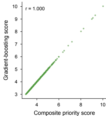
Score concordance
