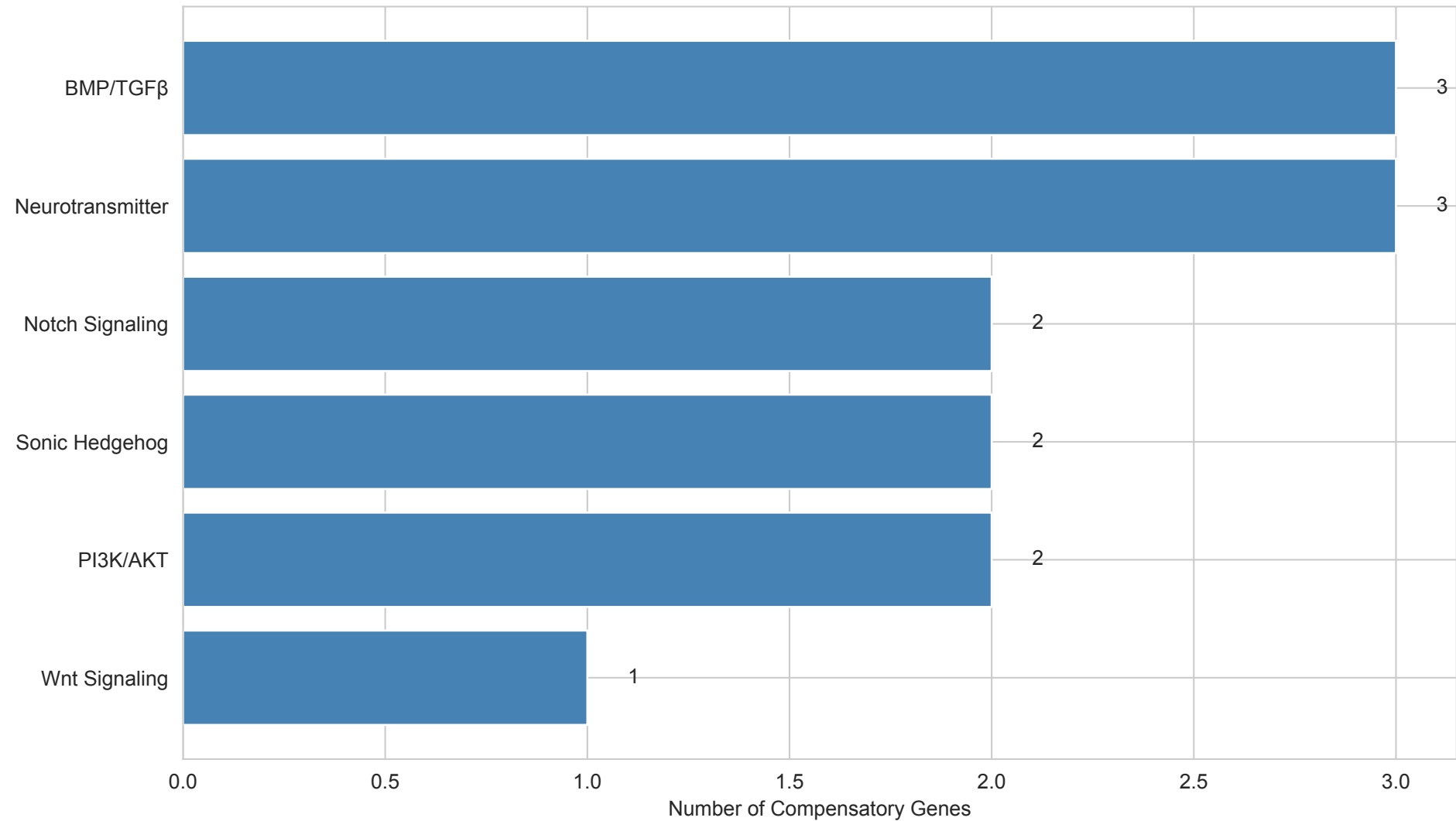
Pathway Enrichment in Compensatory Genes
