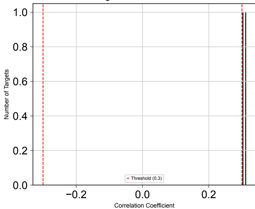
B. Target Correlation Distribution
