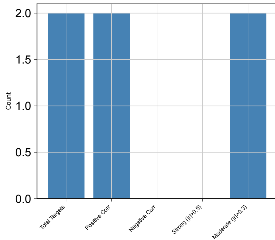
C. Network Statistics
