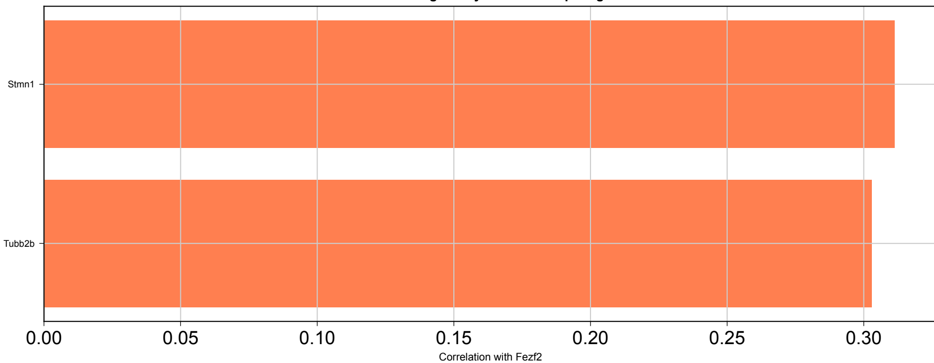
A. Fezf2 Regulatory Network - Top Targets
