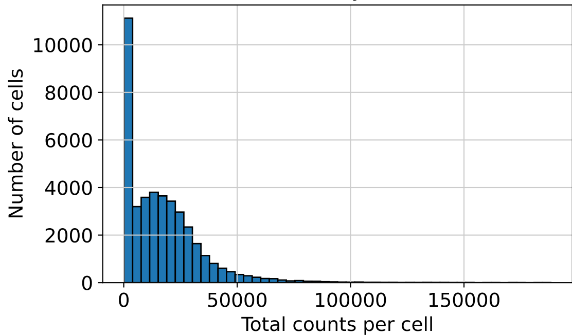
Total Accessibility Distribution
