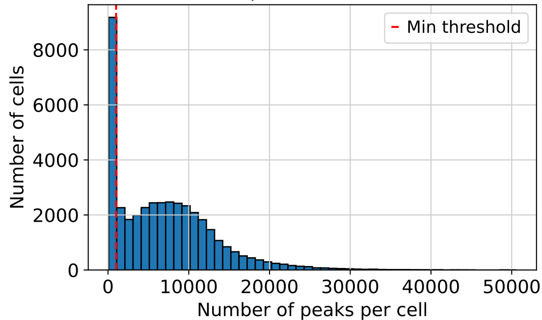
Peaks per Cell Distribution
