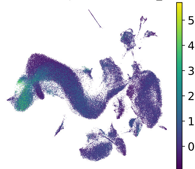
Subcerebral Projection Neurons_score
