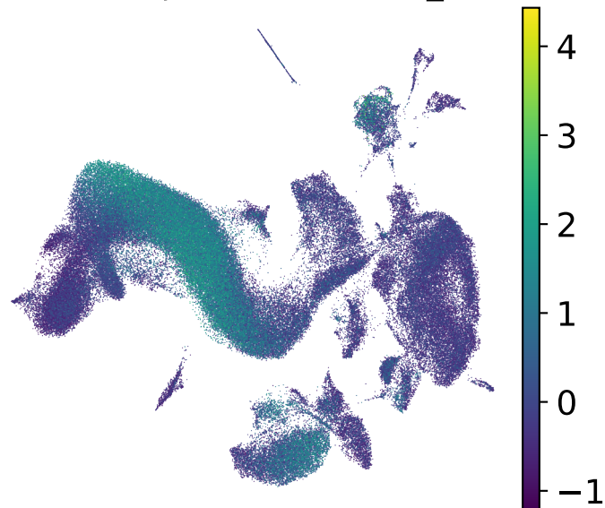
Callosal Projection Neurons_score
