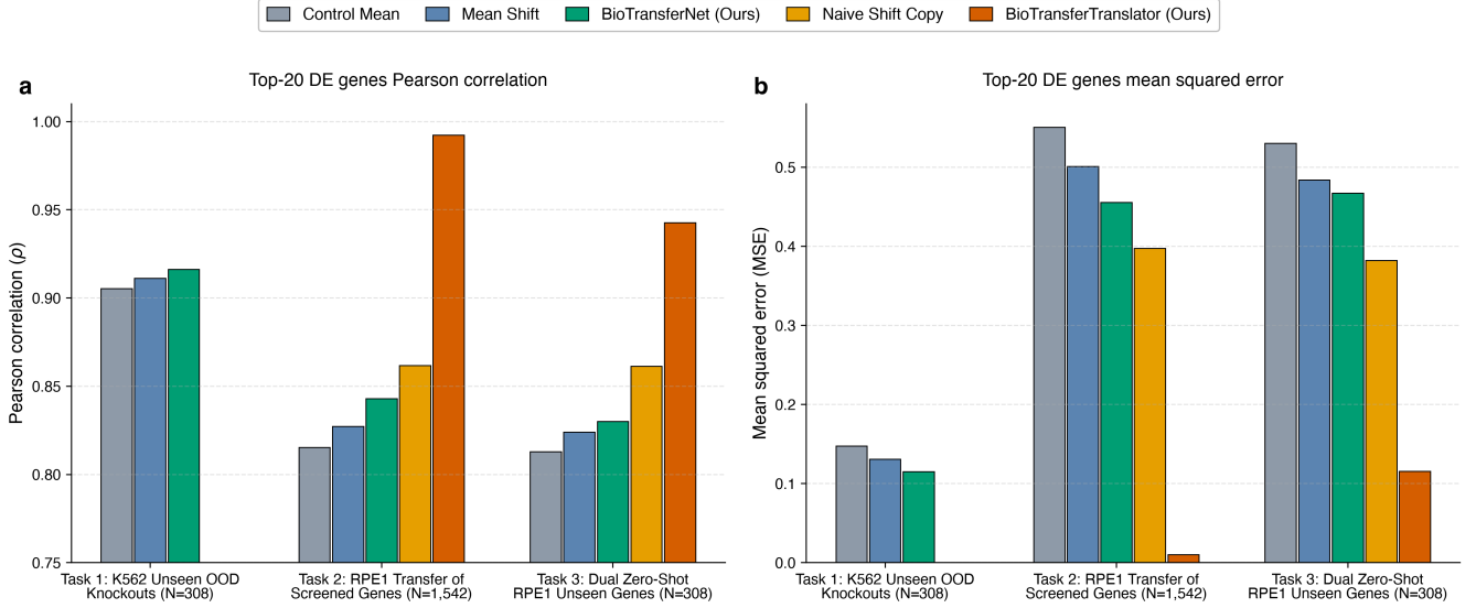
Figure 1: BioTransfer cross-cell benchmark performance across evaluation tasks. a , Pearson correlation ( \rho ) on the top-20 differentially expressed (DE) genes across: Task 1 (K562 unseen OOD knockouts, N = 308 ), Task 2 (RPE1 transfer of screened genes, N = 1,542 ), and Task 3 (Dual zero-shot RPE1 unseen genes, N = 308 ). b , Mean squared error (MSE) on top-20 DE genes across all three tasks. BioTransferTranslator achieves a 69.8% error reduction on unseen test targets compared to naive shift copying.
