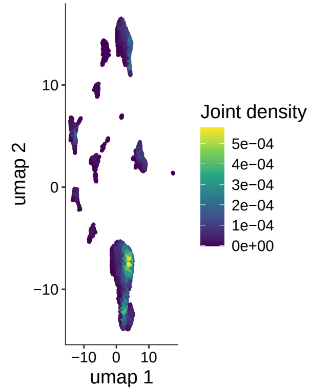
Cdkn1a+ Ccnd1+
