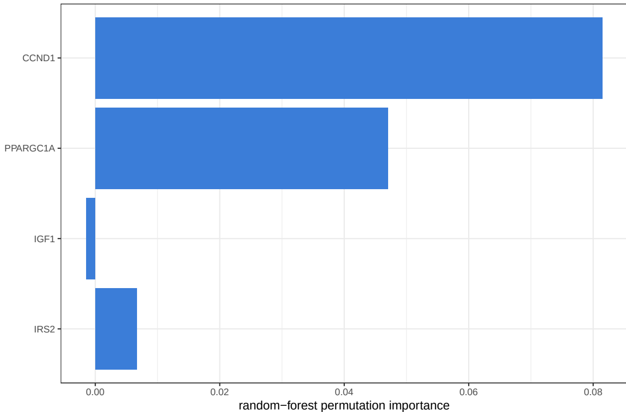
D Random-forest importance
