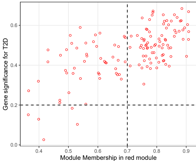
Module membership vs. gene significance cor=0.64, p=3.8e-17
