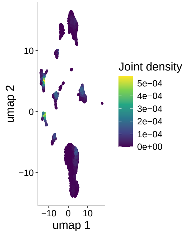
Ppargc1a+ Ccnd1+
