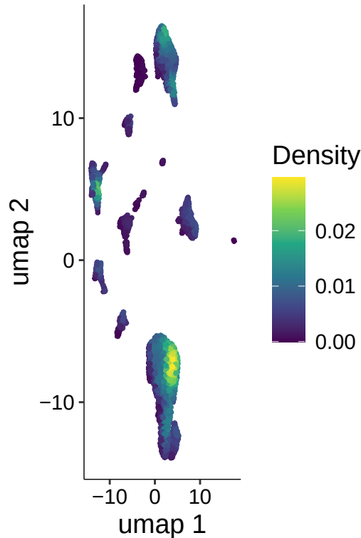
Ccnd1
