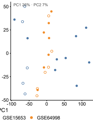
ComBat
