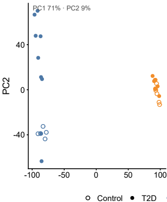
Uncorrected
