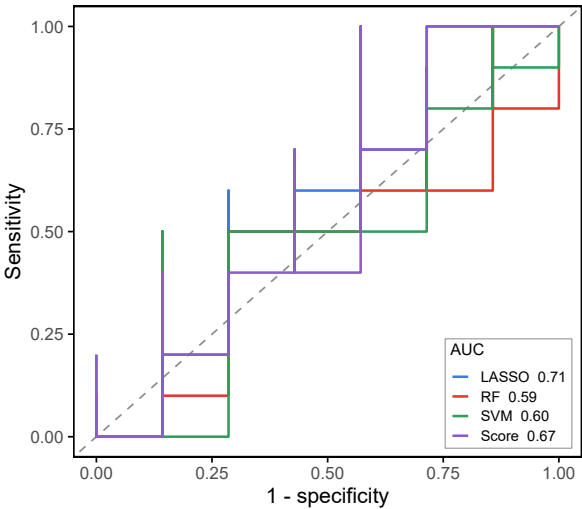
GSE23343 (independent)
