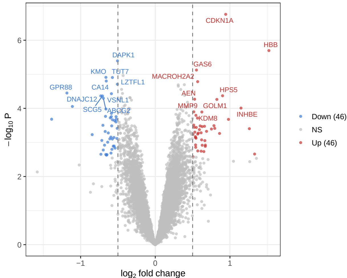
C1: Obese T2D vs Lean (limma, dataset covariate)
