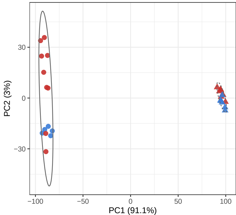
Before batch correction
