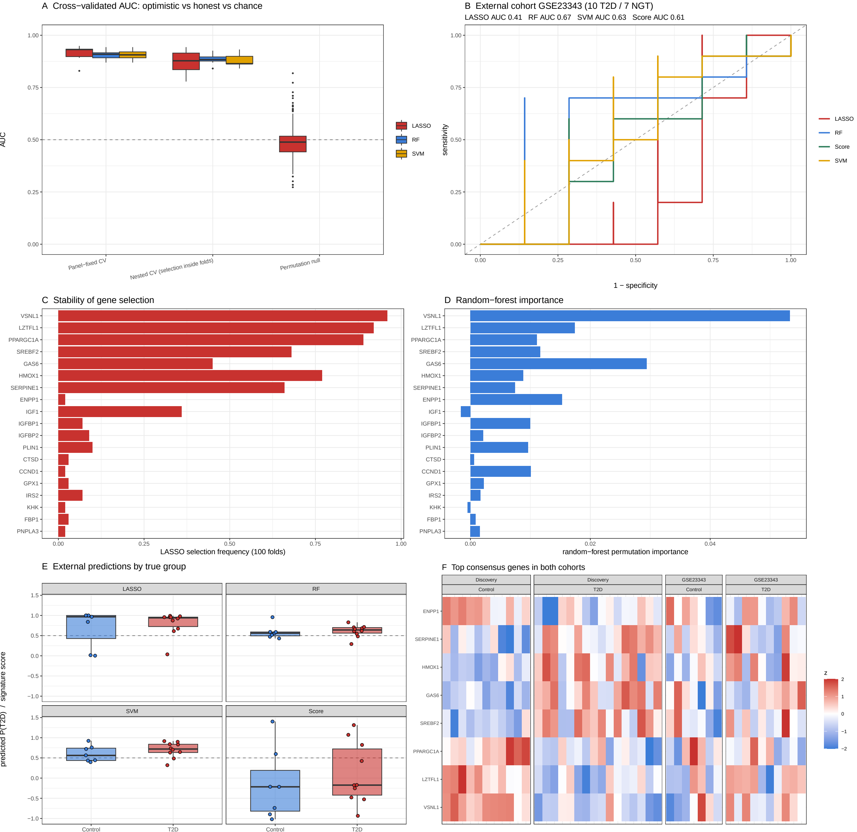
Fig 4 Machine-learning evaluation of the candidate panel Discovery: 27 samples (16 T2D / 11 lean), 19-gene panel. External: GSE23343 (10 T2D / 7 NGT). Permutation P = 0.00498
