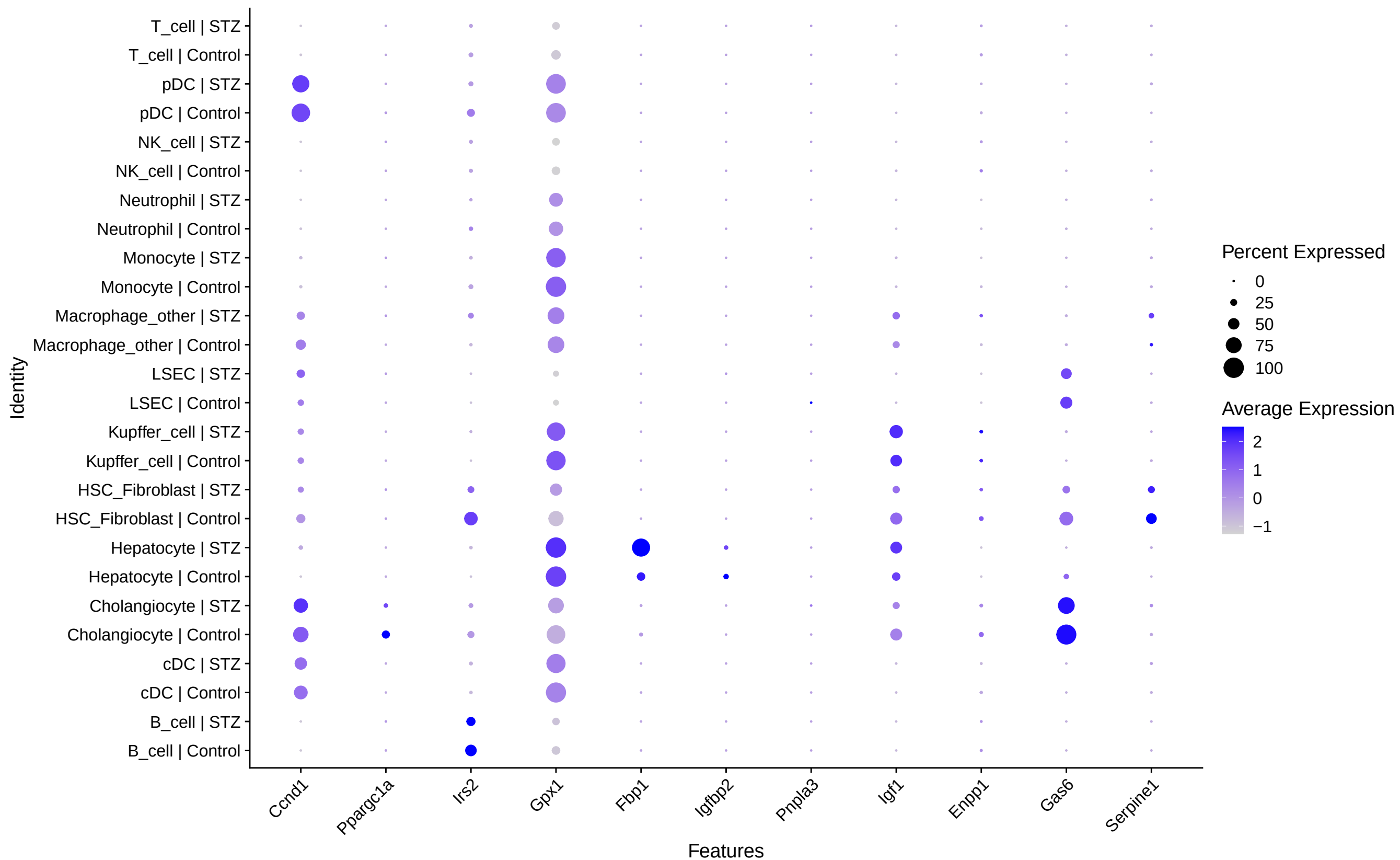
liver – top candidates by cell type and condition
