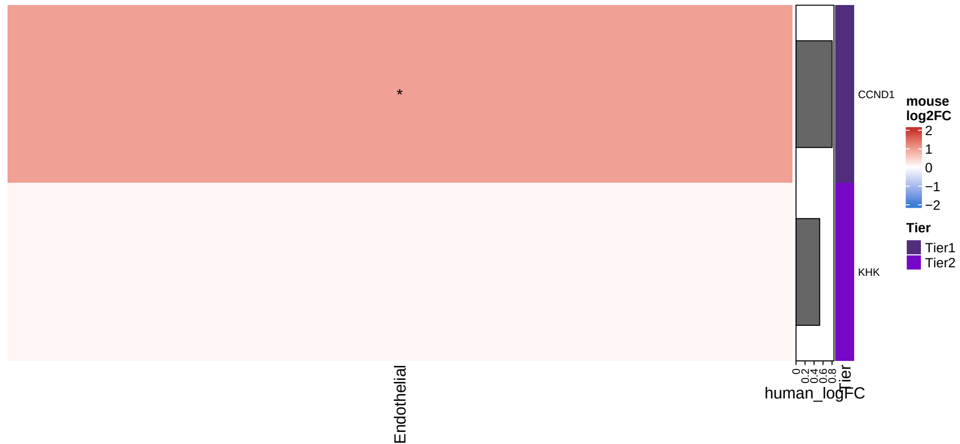
kidney – STZ vs Control pseudobulk logFC for human bulk candidates (* FDR<0.05)
