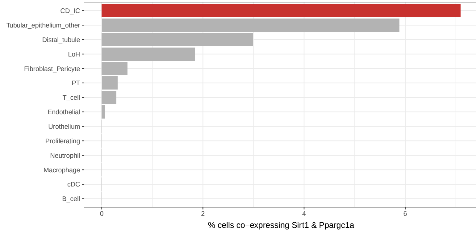
kidney – AMPK axis
