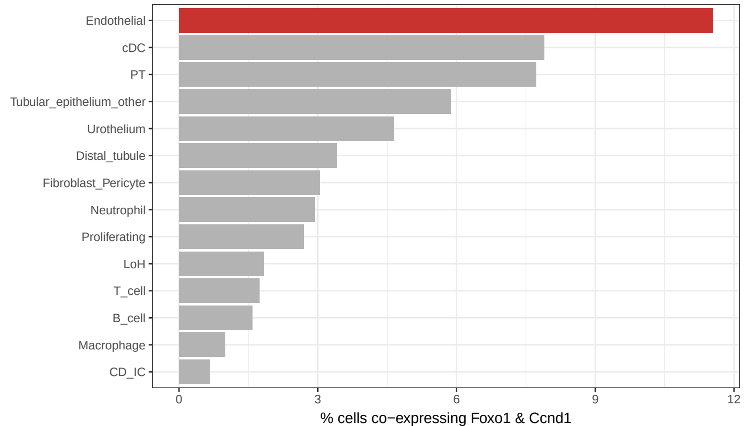
kidney AMPK axis
