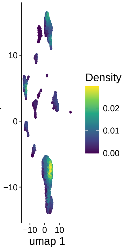
Ccnd1
