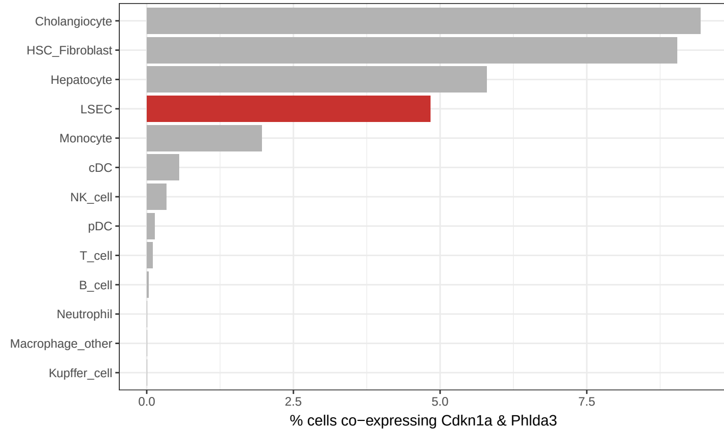
liver p53 axis
