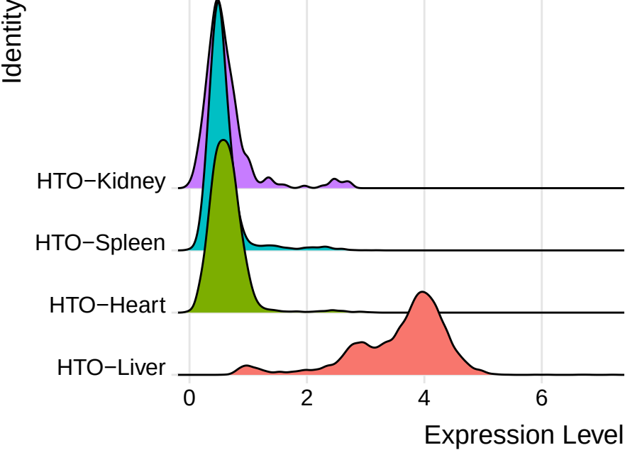
HTO-Liver
