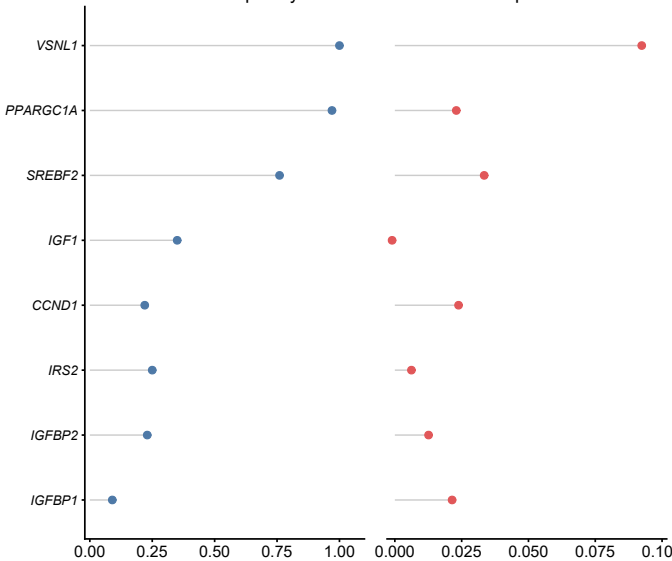
LASSO frequency
