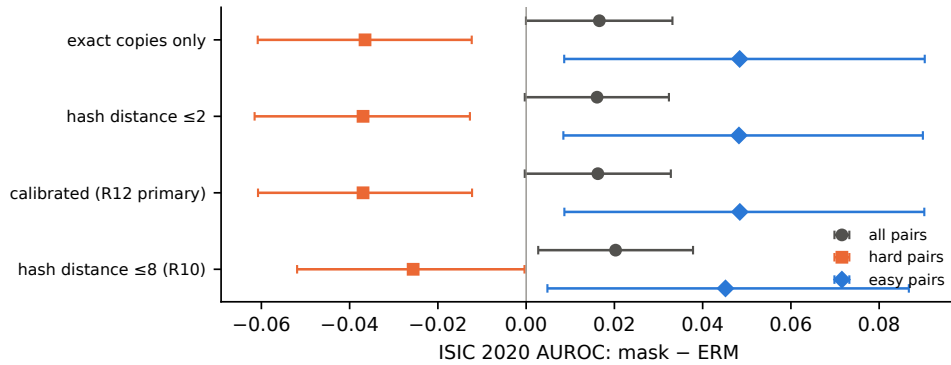
Figure 6: ISIC 2020, mask – ERM on all, hard and easy pairs under four duplicate rules (crossed 95% CIs).
