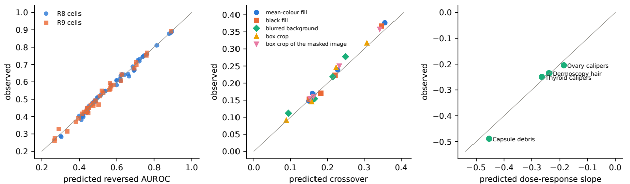
Figure 7: Prospective test of the theory. Left: predicted versus observed reversed AUROC for every R8 and R9 cell. Middle: R8 crossovers. Right: R9 dose-response slopes. Grey lines are the identity.
