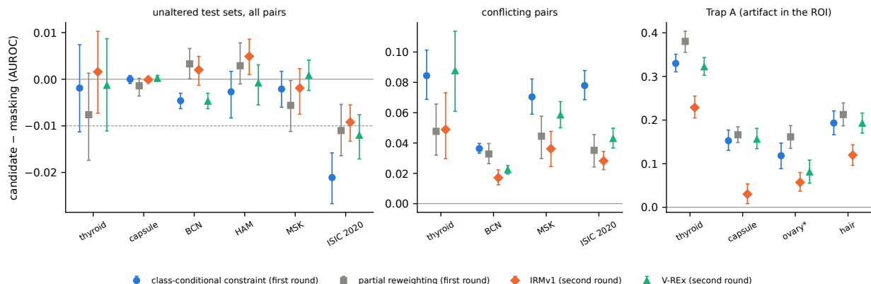
Figure 6: The four candidates closest to dominating masking, each minus masking (AUROC, crossed 95% CIs), on the confirmation data of their registered round (first round: class-conditional constraint, partial reweighting; second round, on new resamples: IRMv1, V-REx). Left: all pairs of the unaltered test sets (dashed: the registered margin -0.01 ). Middle: shortcut-conflicting pairs. Right: Trap A, the worse of reversed and correlated AUROC; *ovary held out from every choice.
