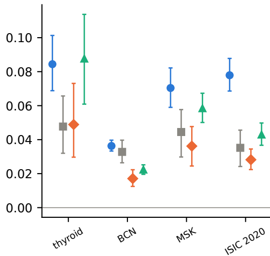
conflicting pairs
