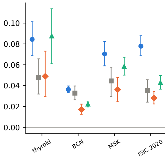
conflicting pairs
