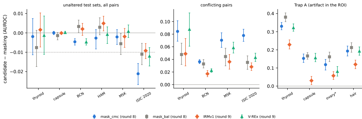
Figure 29: The four best candidates minus masking (crossed 95% CIs). Left: all pairs of the unaltered test sets (dashed: the registered margin -0.01 ). Middle: conflicting pairs. Right: Trap A min(reversed, correlated); *ovary held out from every choice.
