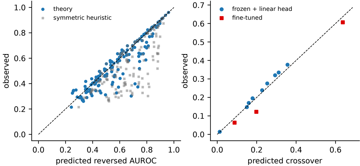
Figure 3: Left: predicted versus observed reversed AUROC (theory, blue; symmetric heuristic, grey). Right: predicted versus observed real-trap crossover (frozen encoders, blue; fine-tuned, red).
