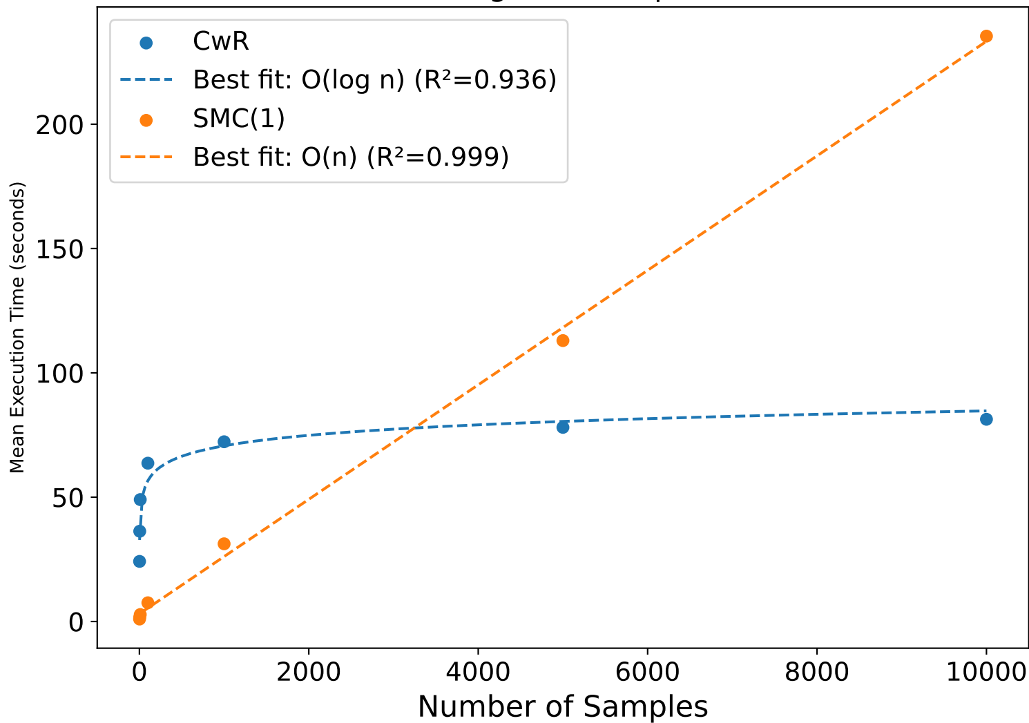
Execution Time Scaling with Sample Size ( N_e \cdot L = 10^{12} )
