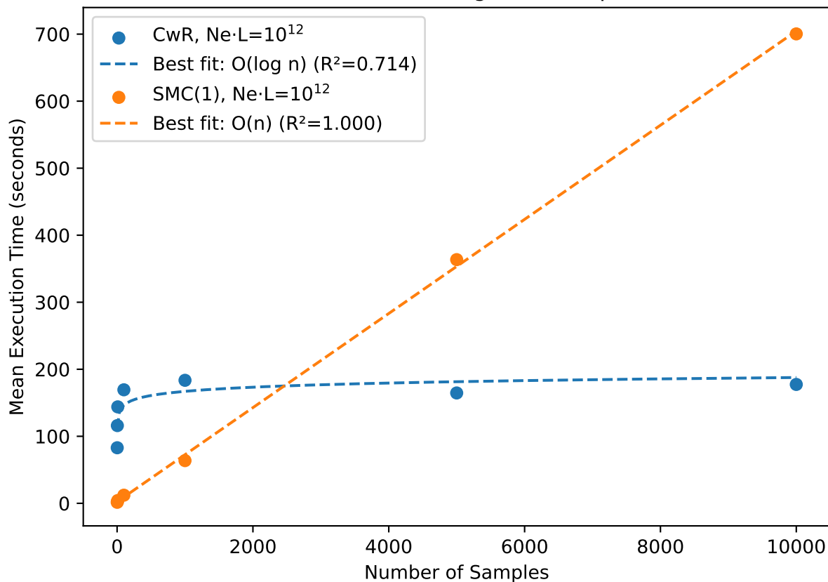
Execution Time Scaling with Sample Size
