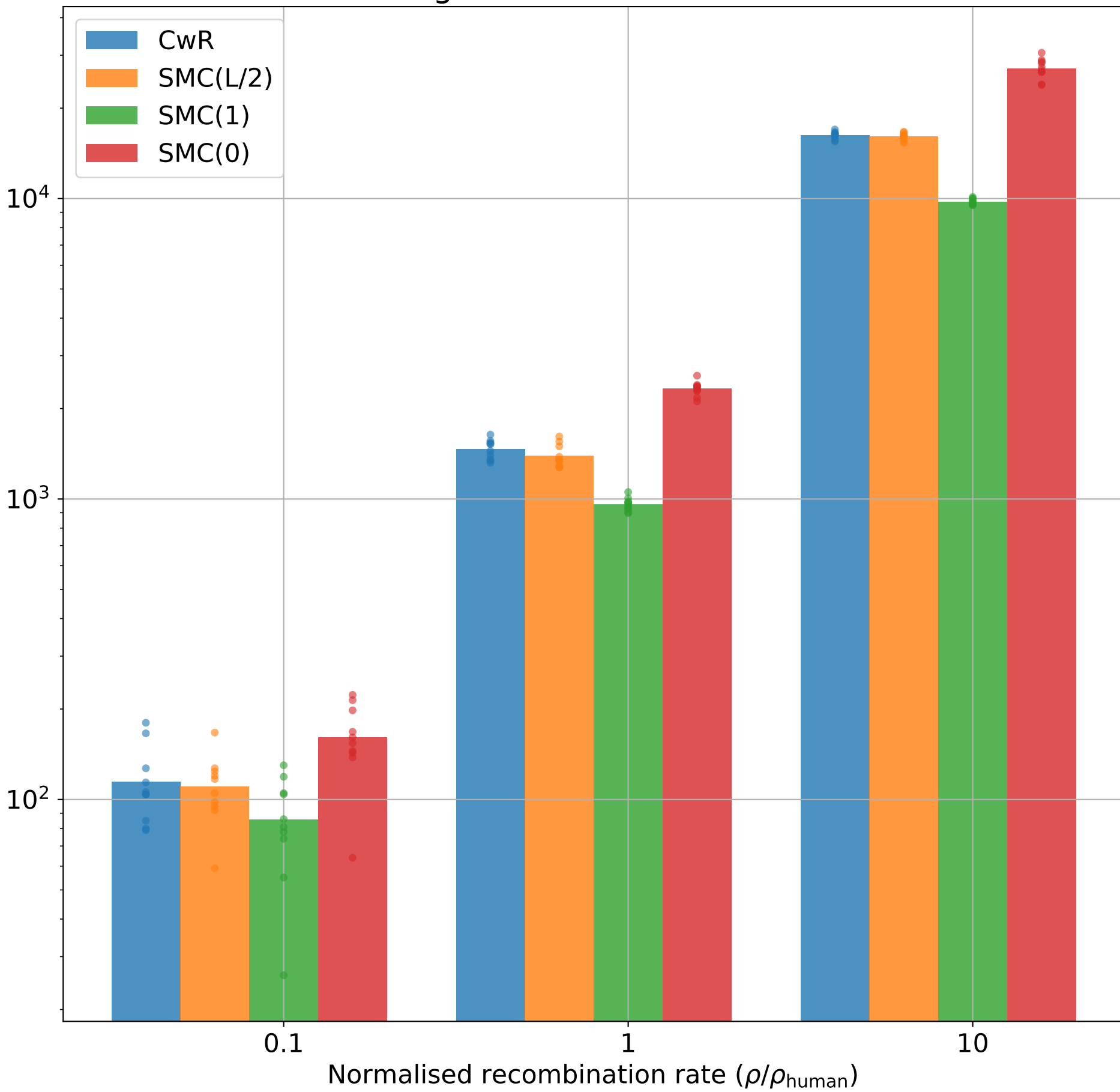
Number of trees making the ARG
